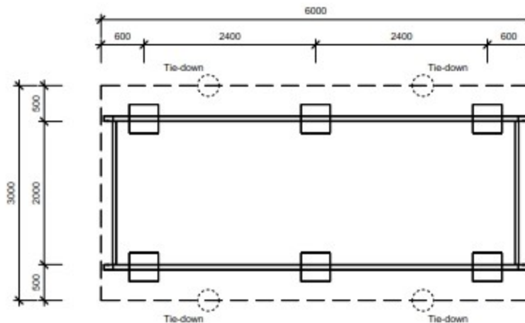
1 Footing Layout 1 : 50
